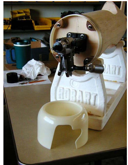
Mount engine on firewall & cut & fit cowling
